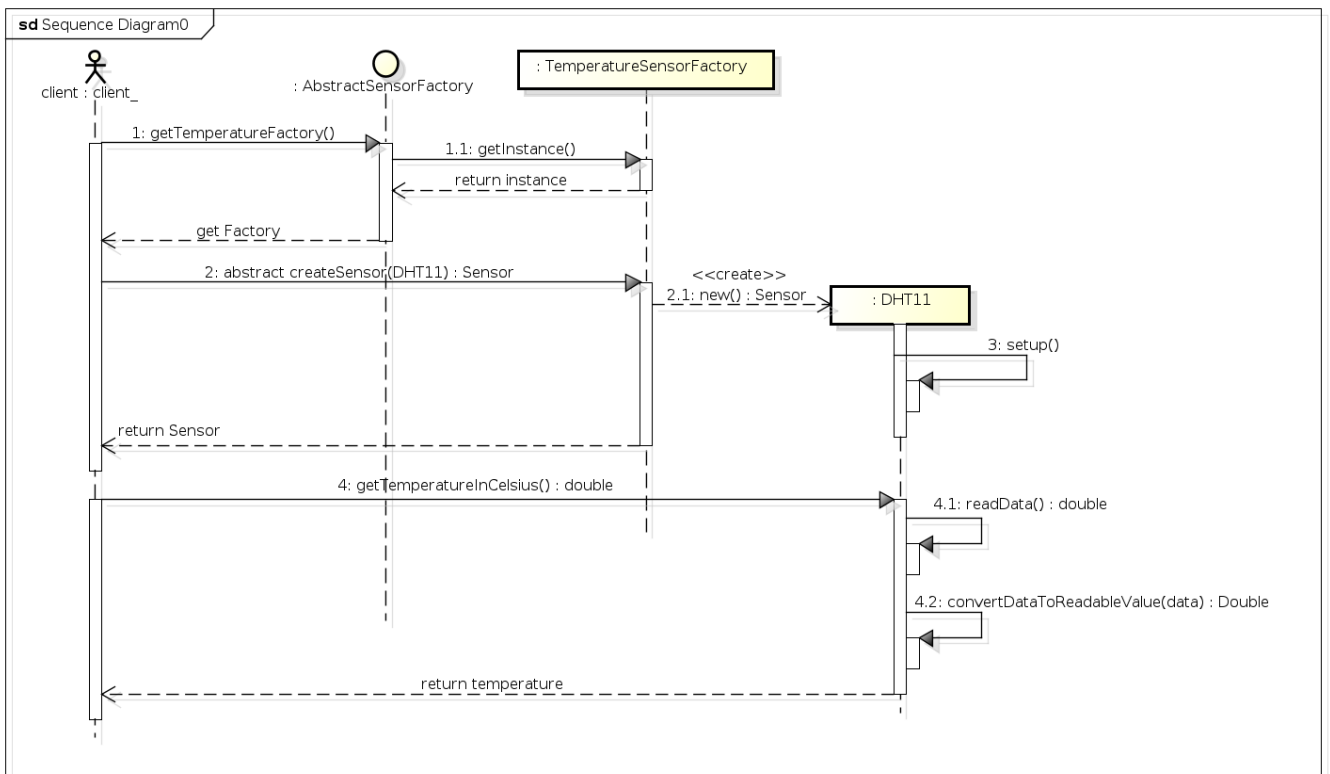
Figure 12: Sequence diagram
