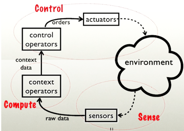
Figure 11: Sense-Compute-Control environment[10]
