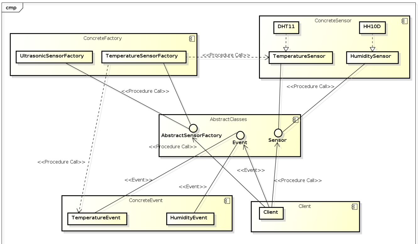
Figure 13: LibsensorPy’s structural view
